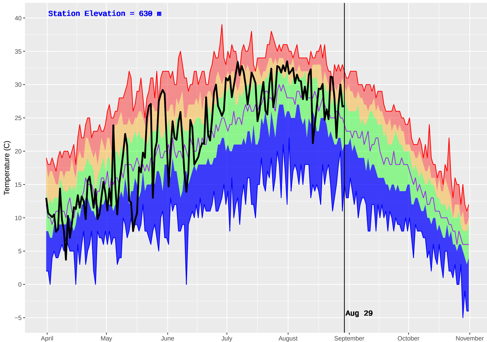
GRAND FORKS (392) : Historical (1981–2016) and Current (2017) Noon Temperature
